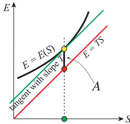
Figure 18.1: Legendre 変換
